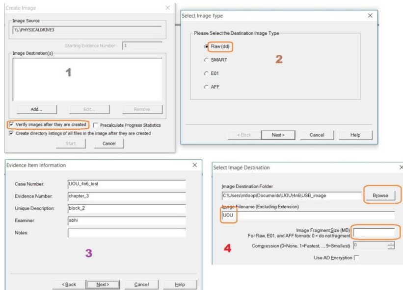
Figure 46: Steps to demonstrate the imaging of the disk
