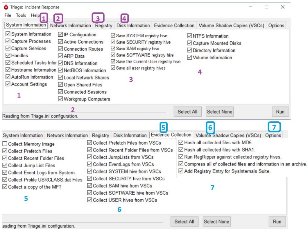
Figure 41: Triage_IR tool
