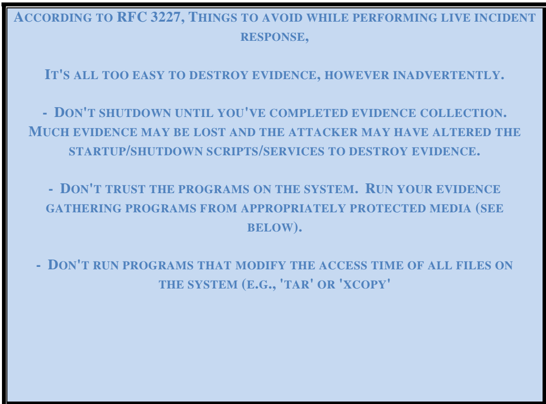
Figure 36: RFC 3227 guidelines for live incident response
