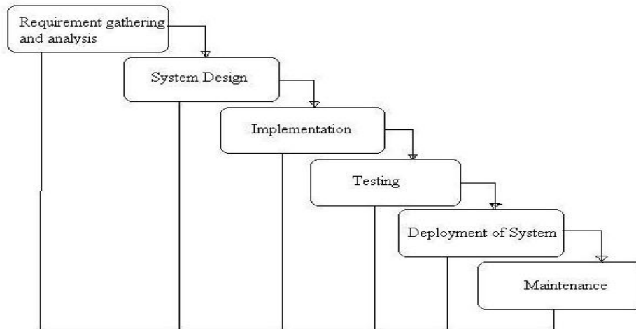
Figure 6 : Waterfall model
