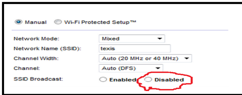
Figure 18: SSID settings
