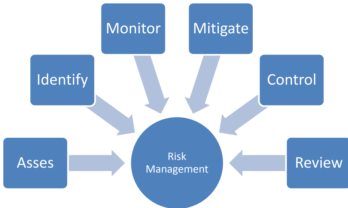
Figure 2: Risk management
