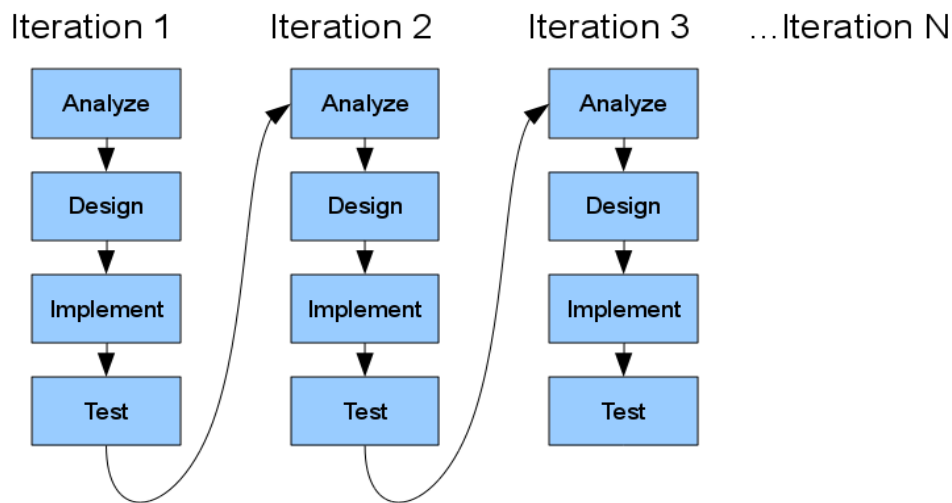
Figure 7: Iterative Model
