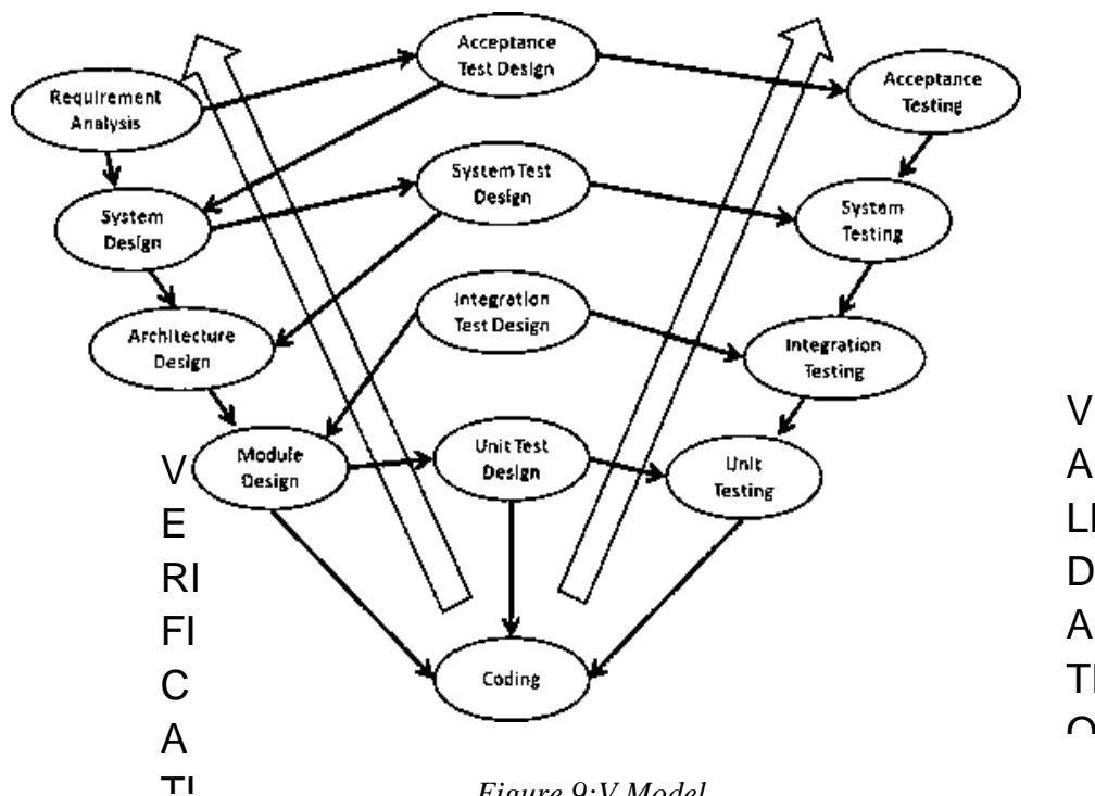
Figure 9:V Model
