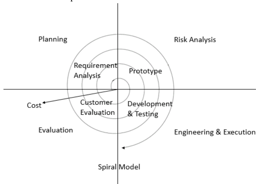
Figure 8: Spiral Model
