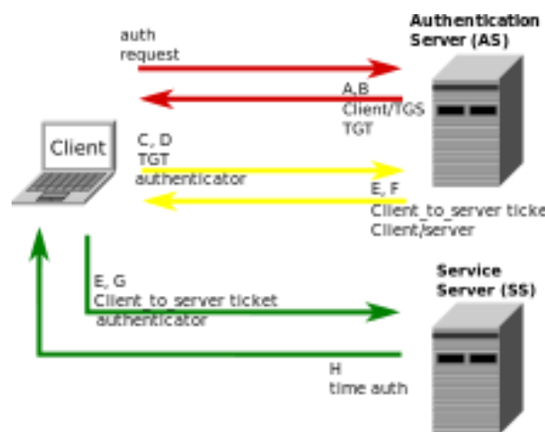
Figure 14: Kerberos Negotiations
