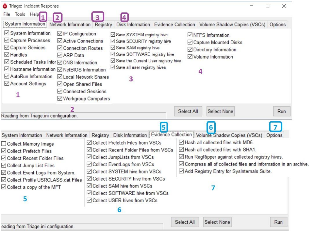
Figure 41: Triage_IR tool
